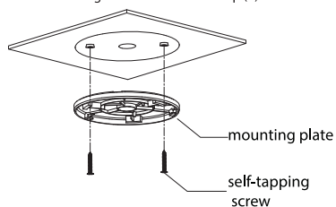
Figure 4-4 Installation step (1)
