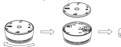
Figure 6-1 Battery replacement
