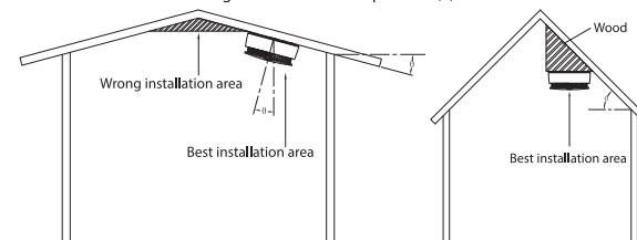
Figure 4-3 Installation position (2)
