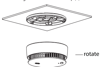
Figure 4-5 Installation step (2)
