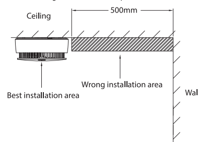
Figure 4-2 Installation position (1)
