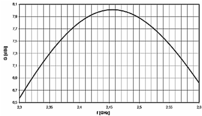
The antenna gain as a function of frequency.
