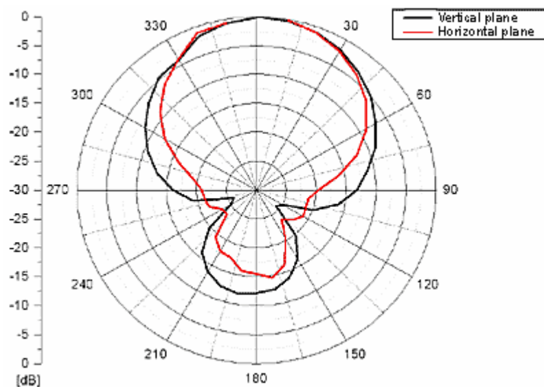
Radiation characteristic in V (black) and H (red) vector plane.
