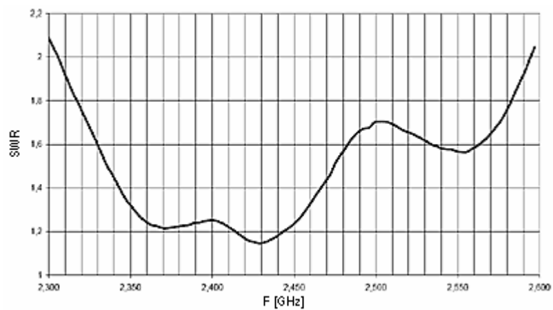
Standing wave ratio characteristic in the frequency function.
